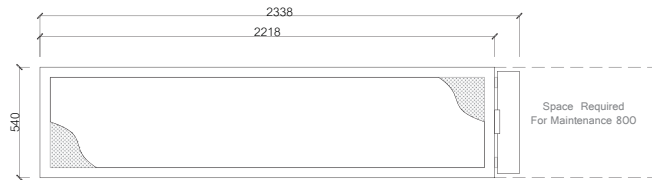
End View
