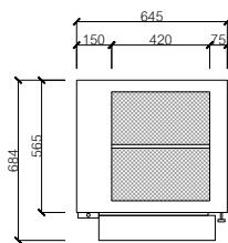
Plan View
