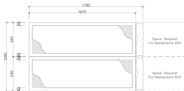
End View
