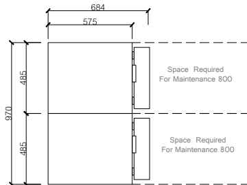
End View
