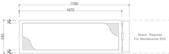
End View
