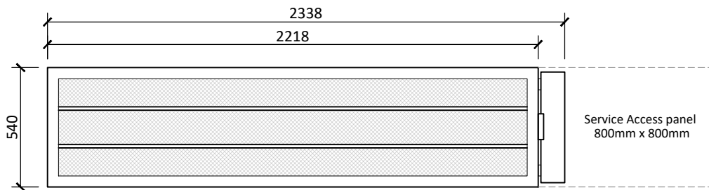
END VIEW
