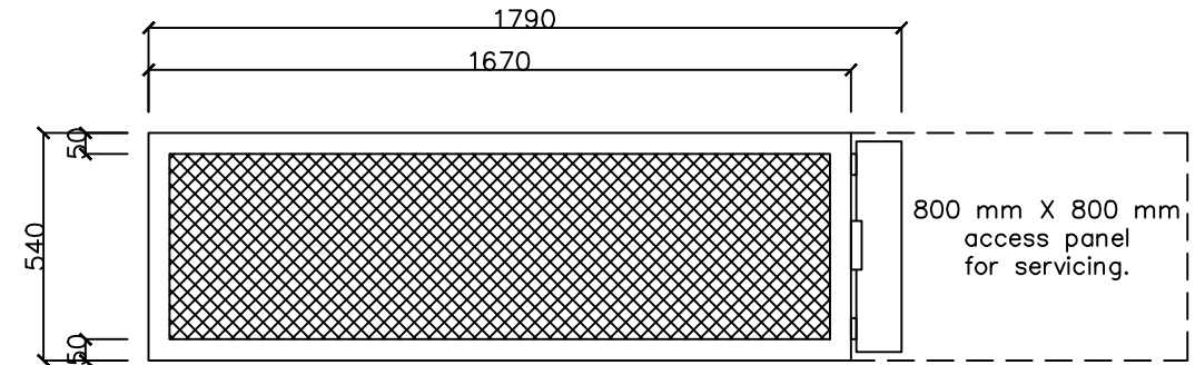
③ END VIEW (INLET) Scale 1:20@A3
