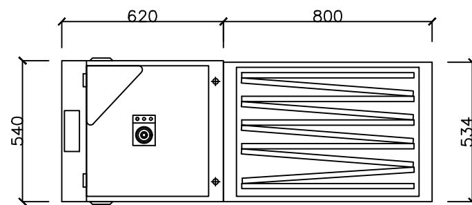
② FRONT VIEW Scale 1:20@A3
