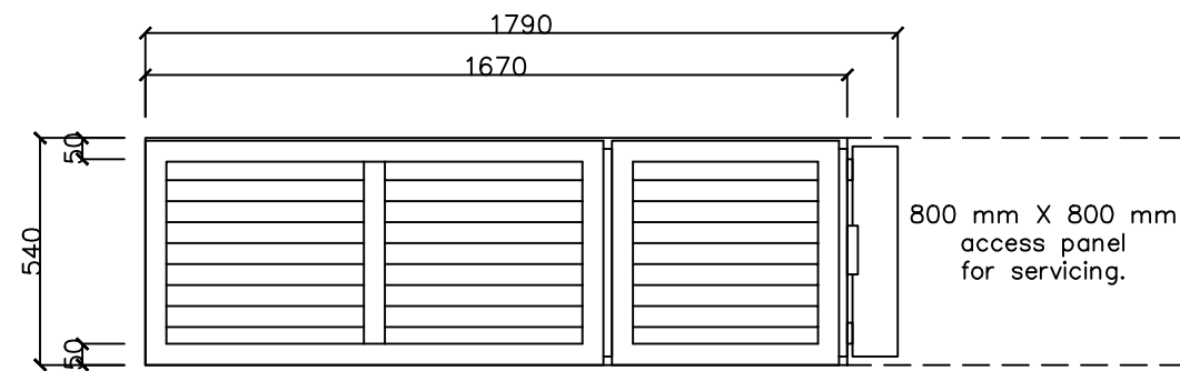
④ END VIEW (OUTLET) Scale 1:20@A3
