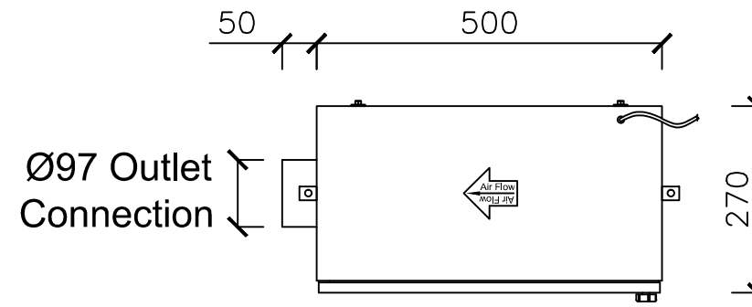
① TOP VIEW Scale 1:10 @ A3
