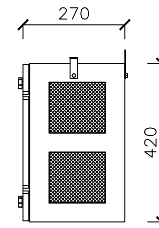
④ SIDE VIEW Scale 1:10 @ A3
